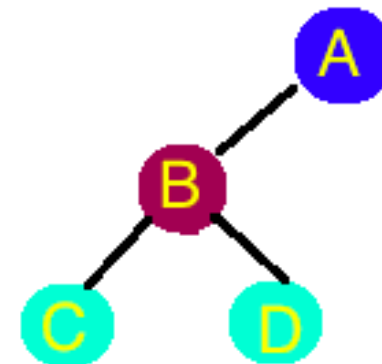
Subgraph 2
