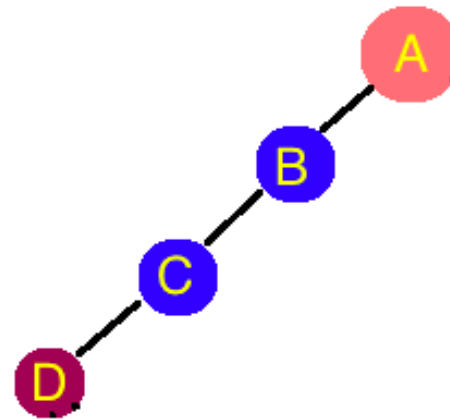
Subgraph 1
