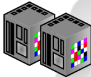
OpenStack Compute
